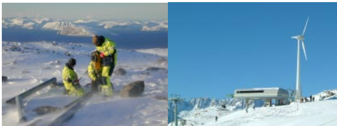
Figure 4 Foundation work in connection with site measurement campaign (photo: Kjeller Vindteknikk, Norway) and wind turbine at a walking distance from a ski lift in Gutsch. Turbine is equipped with a de-icing system. (photo: ENCO AG, Switzerland).
